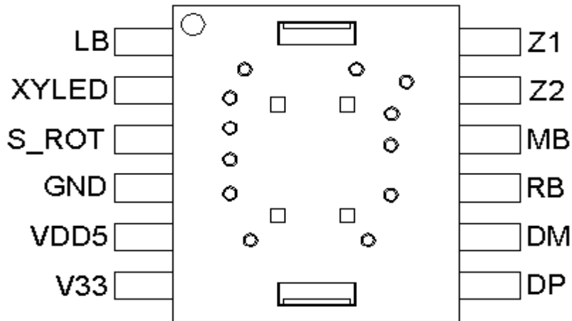
Chart 1 Pin Assignment
